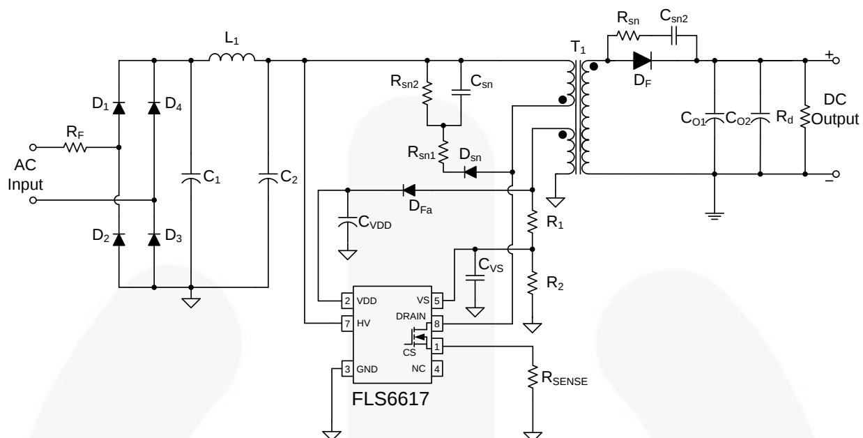
Figure 2. Typical Application
