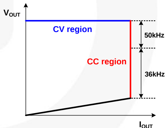
Figure 26. Operation Area
